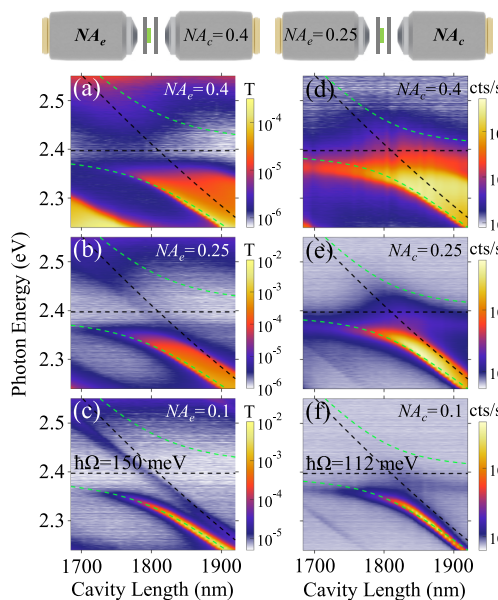
Figure 5. (a–c) Transmittance and (d–f) photoluminescence spectra of the \text{CsPbBr}_3 -cavity system as a function of the cavity length, for a shorter cavity than in Figures 2 and 3. The horizontal dashed black lines indicate the exciton energy, and the tilted dashed black lines indicate the energy of the q = 7 longitudinal cavity mode. The green dashed lines in all panels are the eigenvalues of a 2 \times 2 Hamiltonian representing the exciton–photon coupled system. The coupling constant is the only fit parameter, and the result is shown in (c) and (f) for transmittance and photoluminescence measurements, respectively. The coupling was not changed for measurements with different NA .
