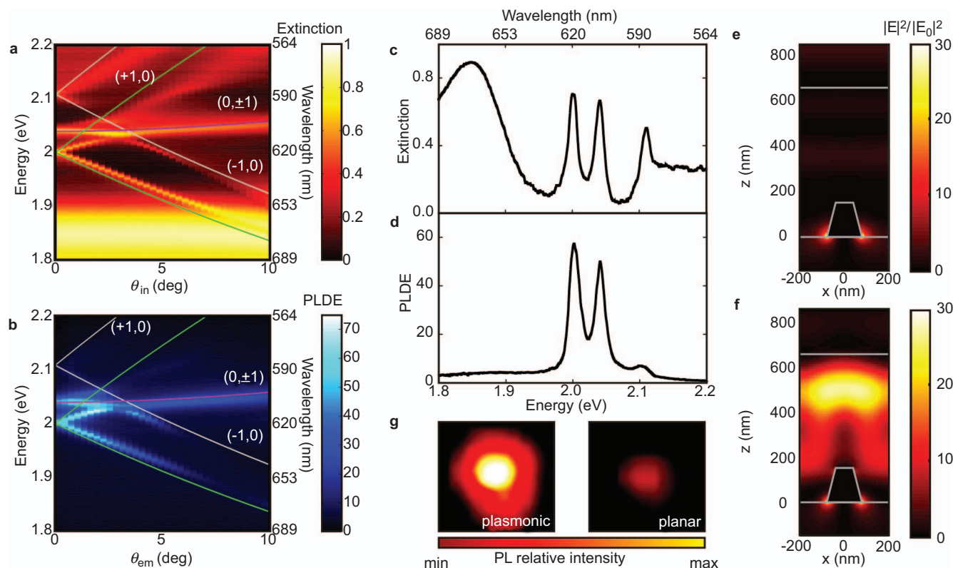
Figure 2 (a) Extinction of p-polarized light as a function of the photon energy and the angle of incidence \theta_{in} of a layer of dye deposited on top of the investigated array of aluminum particles. (b) p-polarized directional emission enhancement as a function of the photon energy and the emission angle \theta_{em} measured on the same structure excited with a 2.76 eV continuous wave laser at \theta_{ex} = 0^\circ . Gray, purple and green curves correspond to the Rayleigh anomalies calculated for the beams diffracted in a medium with refractive indexes of 1.47, 1.52 and 1.55, respectively. (c) Extinction and (d) PLDE as a function of photon energy measured at \theta_{in} = 0^\circ and \theta_{em} = 0^\circ . (e, f) Simulated spatial distribution of the near-field intensity enhancement in a plasmonic array of antennas on a substrate covered by a polymer layer. The color plot indicates the intensity enhancement of the plane intersecting the antennas at y=0 in a unit cell of the array. The simulations consider a plane wave incident normal to the array with a photon energy of (e) 1.85 eV and (f) 2.04 eV. The antenna and the different dielectric interfaces are outlined using gray curves. (g) Digital photographs taken from the unpolarized emission from the dye layer deposited on top of the plasmonic structure (left) and from the same layer deposited on a dielectric substrate (right) at \theta_{em} \sim 0^\circ . PLDE, photoluminescence directional enhancement.
